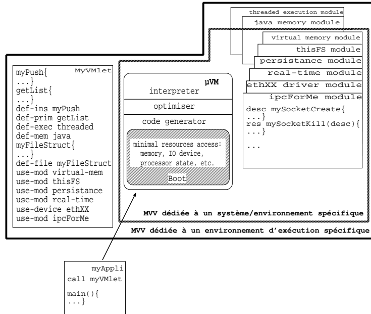
Figure 3: Loading an application.
